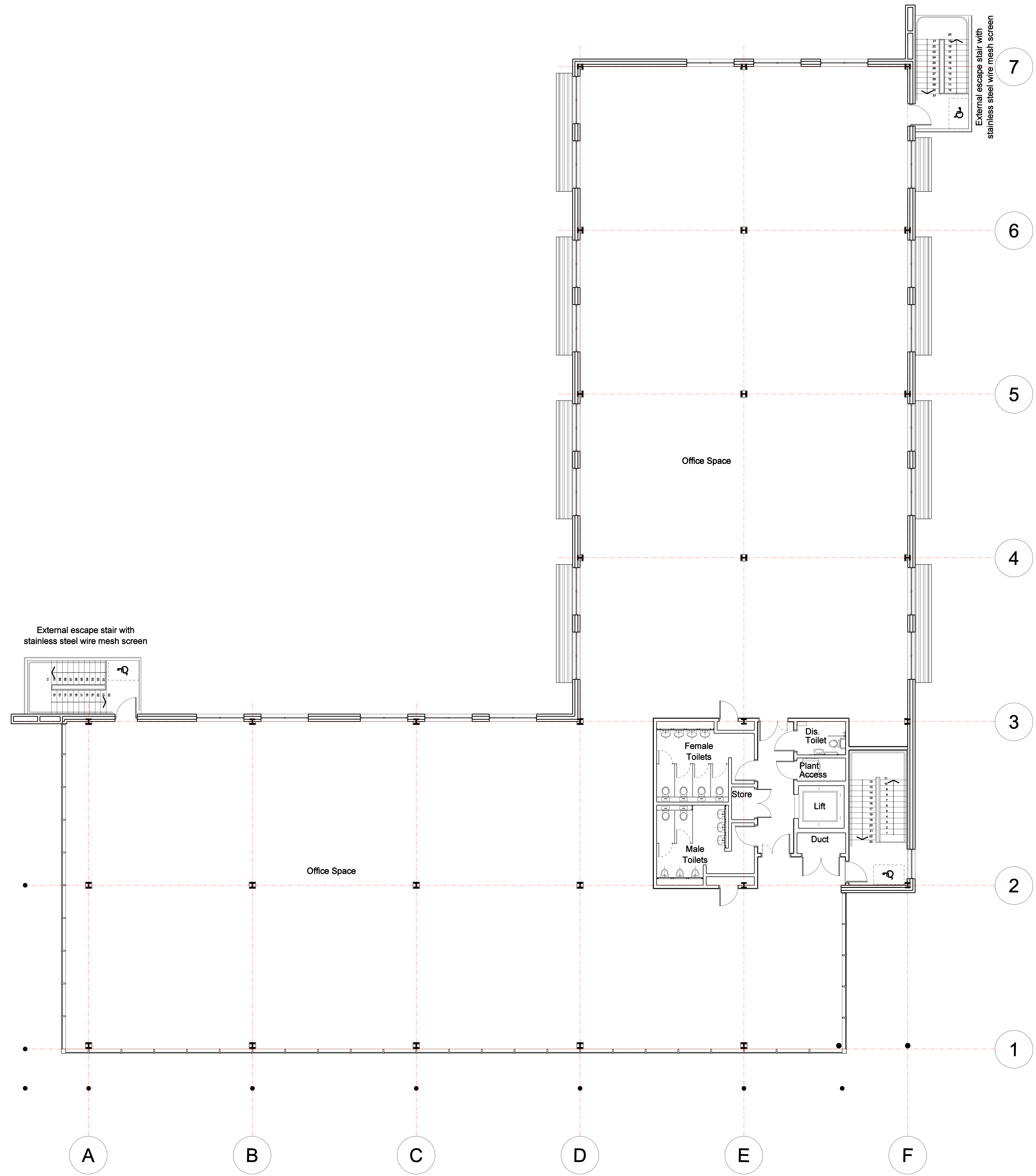
FIRST FLOOR PLAN
